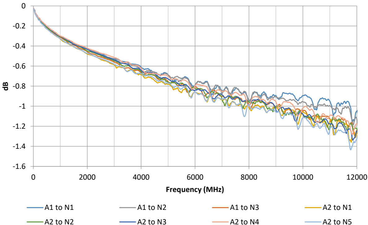
Insertion Loss
