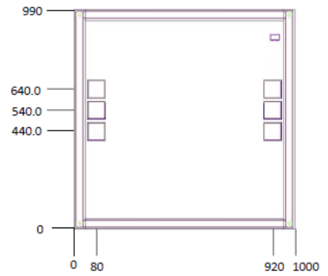
Fig 2. Bonding Pad Positions
