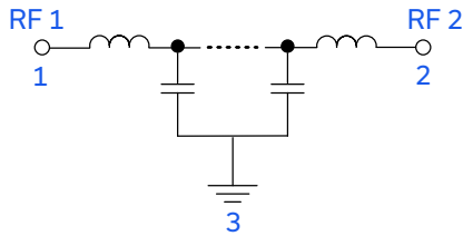
Figure 1. LFCV-3002+ Functional Diagram
