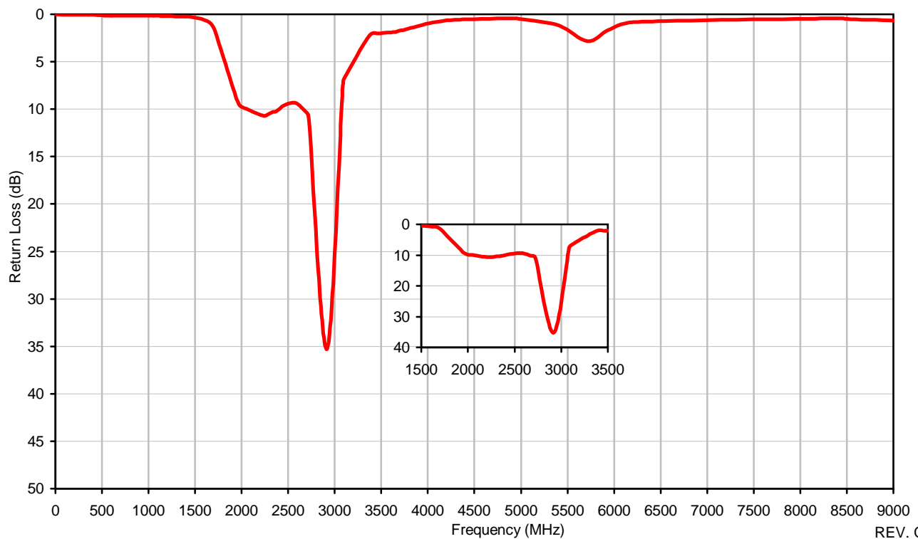
Return Loss
