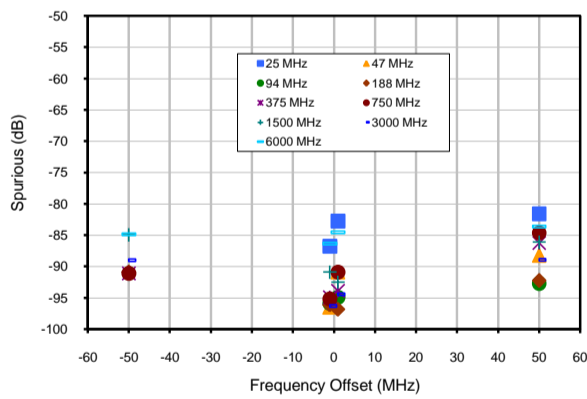
Spurious vs. Frequency Offset (1 & 50 MHz offsets)
