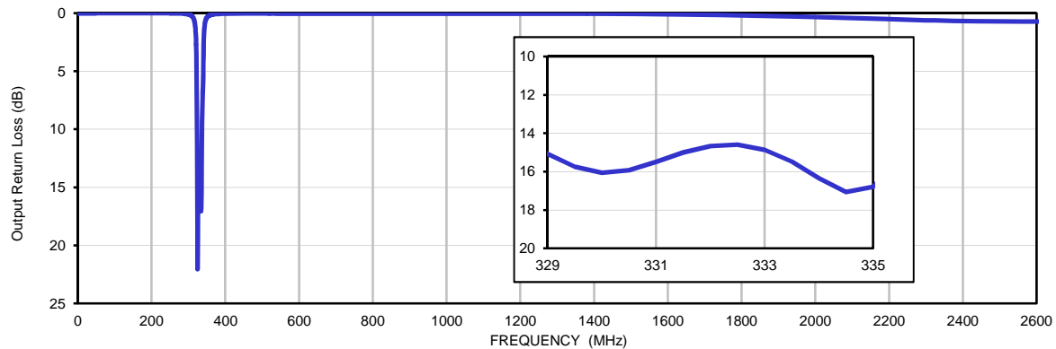
Output Return Loss
