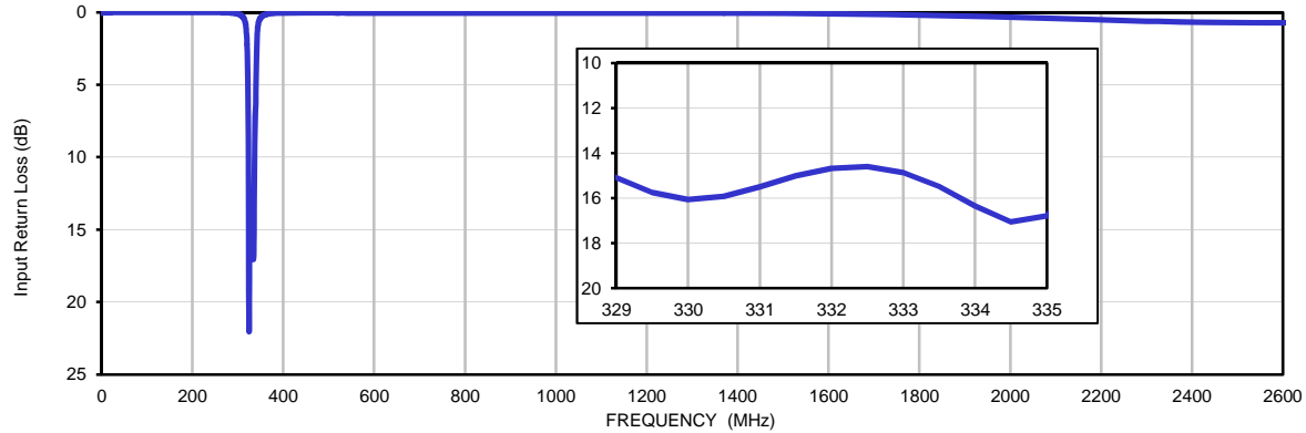
Input Return Loss
