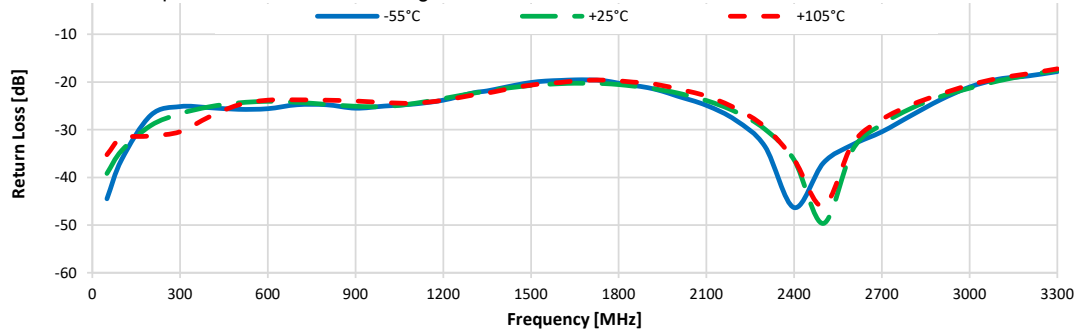
Return Loss Reverse vs. Frequency
